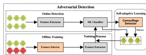
Figure 1: The KuafuDet Framework through Adversarial Detection
